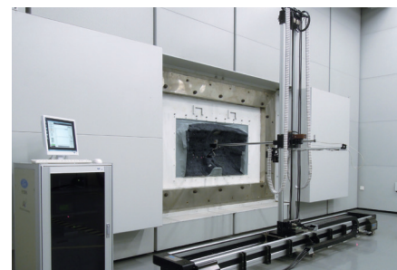
System for evaluation of performances of automotive soundproof materials
